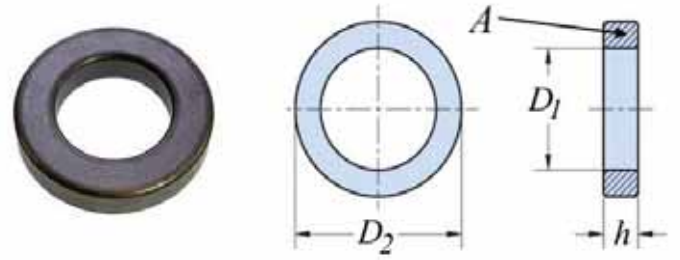
Figure 5 – Annular core dimensions.
