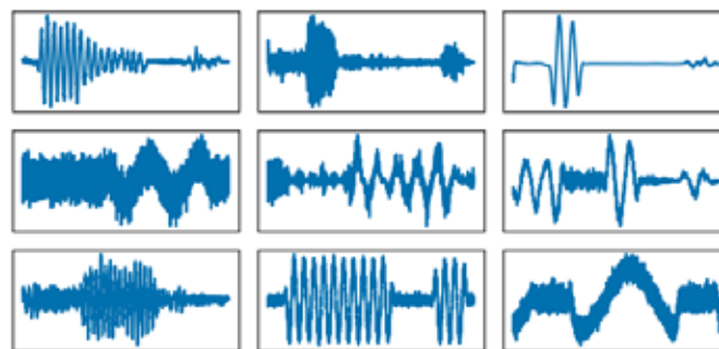
Figure 8 – Good training dataset for the class “Morse code” showing a high variation on different signal impairments, like noise, fading and frequency offsets.
